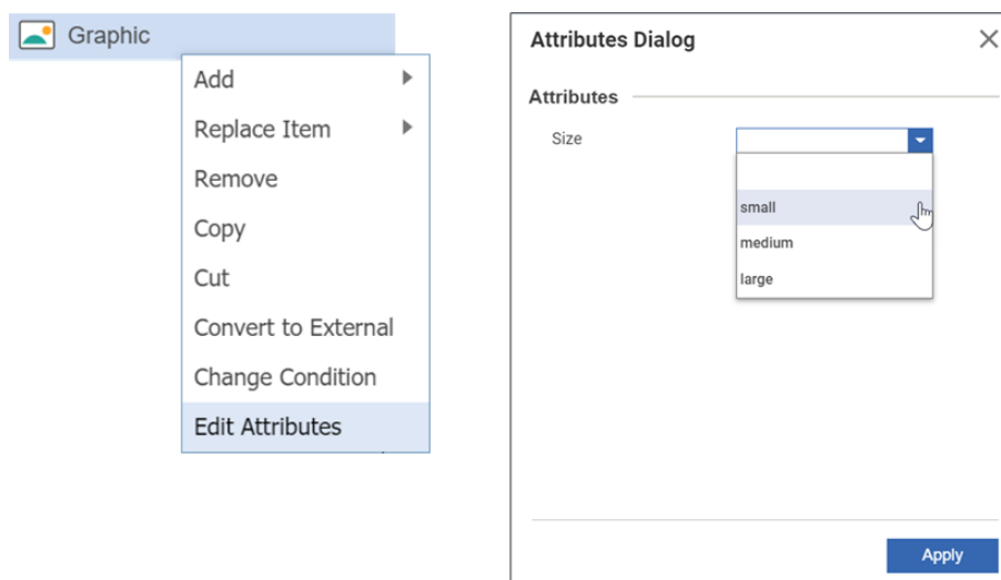
Figure 21: Image Size Attribute Example
