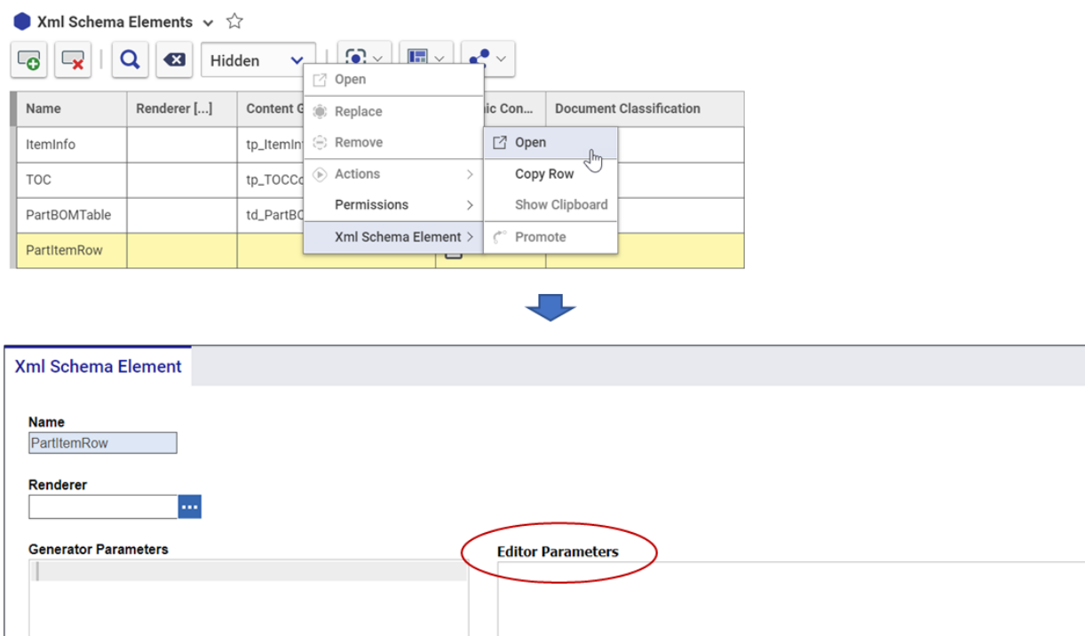
Figure 29: XML Schema Element Form
