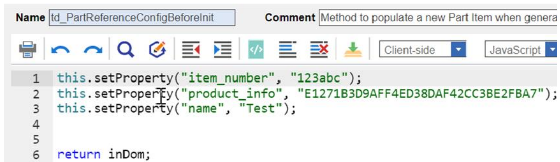
Figure 30: onBeforeInit Method Example
