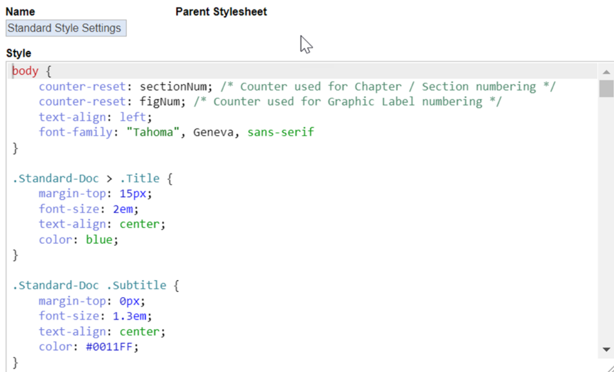
Figure 19: Stylesheet User Interface
