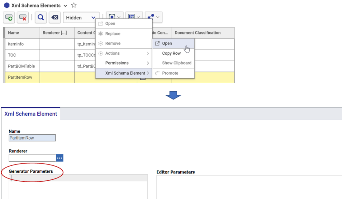
Figure 26: XML Schema Element Form - Content Generator Parameters
