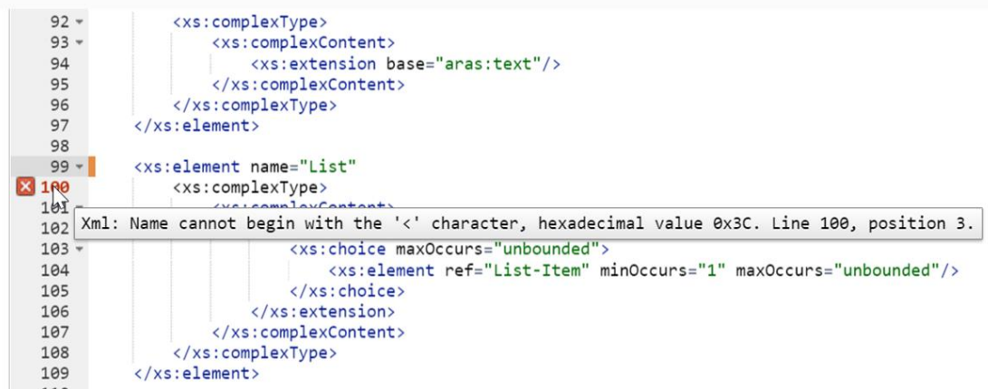
Figure 12: XML Schema Validation Warning
